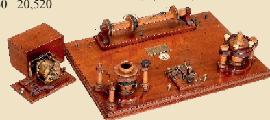
Hughes Induction Balance, W. Groves, London, 1879
